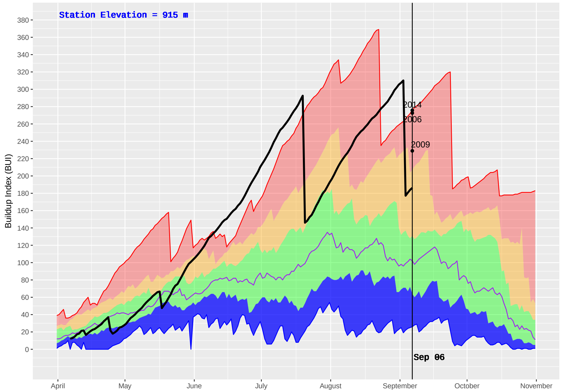
MIDDLE LAKE (226) : Historical (1989–2016) and Current (2017) Noon Buildup Index (BUI)
